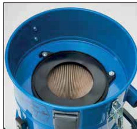
Filter cartridge with 6,000 cm 2 filter surface area
