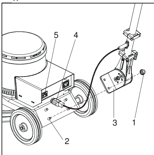
Fig. 5 Assembly of guide bar
