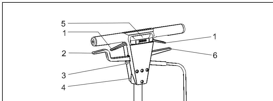
Fig. 3 Switch housing
