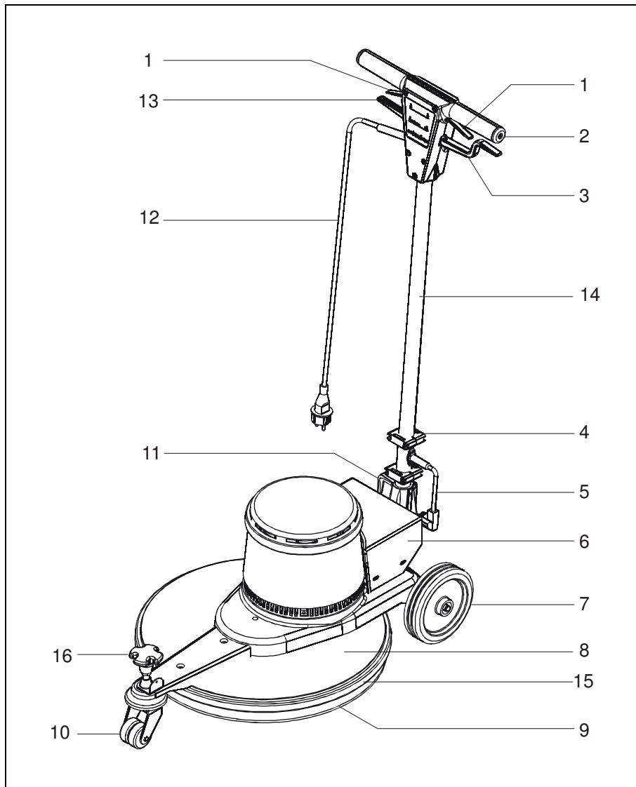
Fig. 1 Appliance overview
