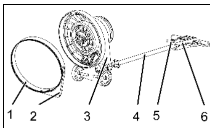
Fig. .: Assembling the vac unit
