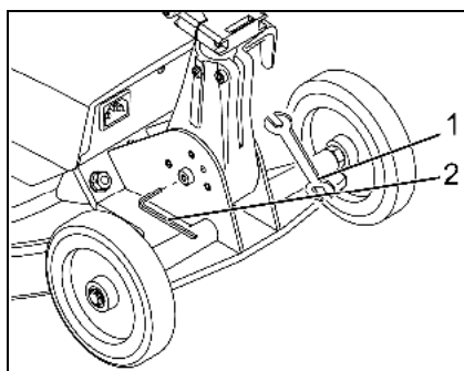
Fig. .: Setting the swivel joint stiffness
