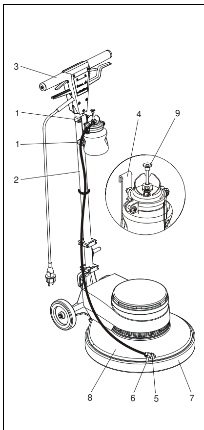
Fig. .: Assembling the spray device
