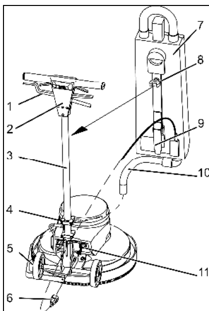
Fig. .: Assembling the suction bin
