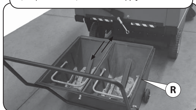
[AKS 85|BM 120 Performance] Machine with manual emptying of the refuse container
