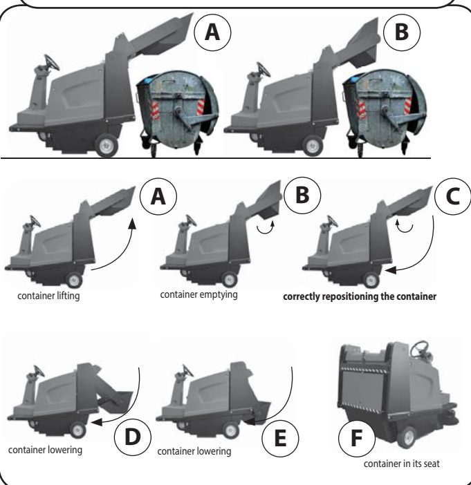
[AKS 85|BM 150H Performance] Machine with hydraulic emptying of the refuse container
