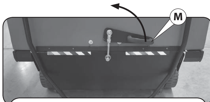
[AKS 85|BM 120 Performance] Machine with manual emptying of the refuse container
